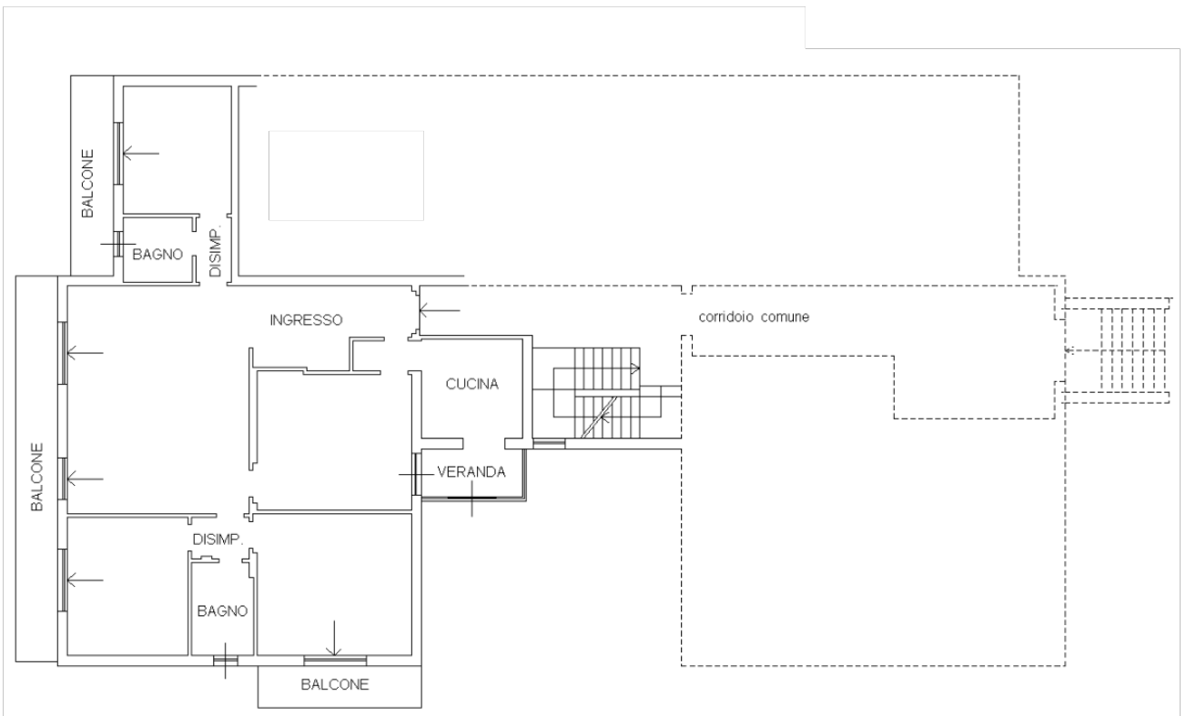
PIANO T H=3,05m
