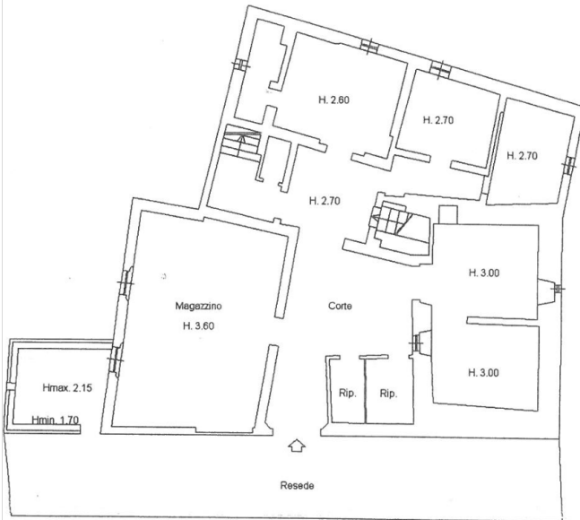
PIANO TERRA
