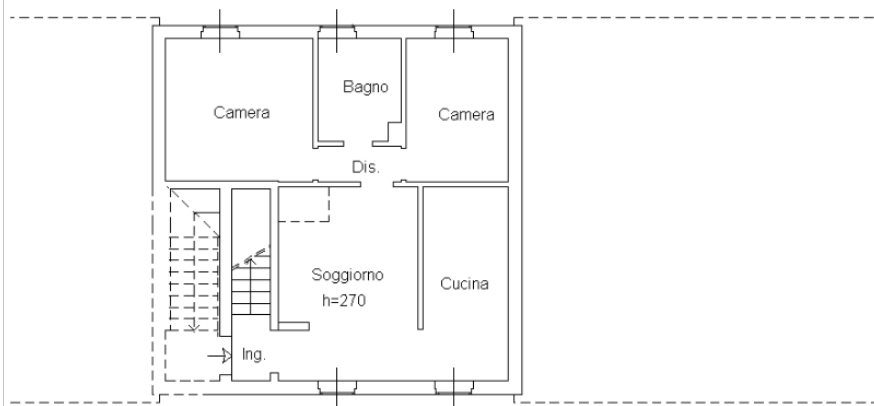
Pianta Piano 2
