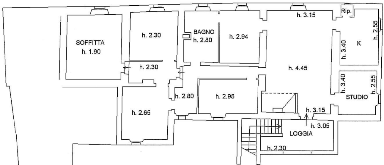
PIANO 1
