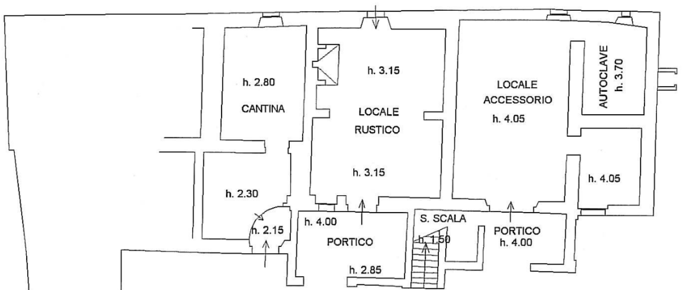
PIANO TERRENO
