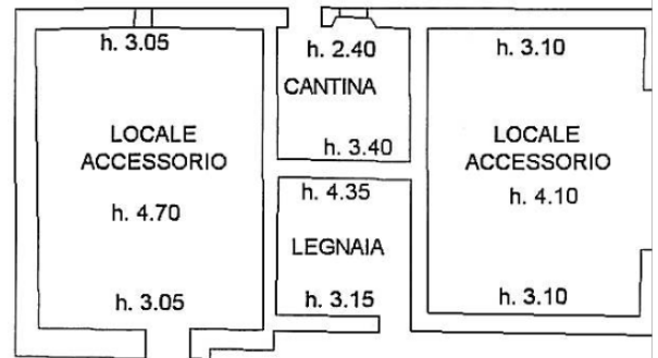
PIANO TERRENO
