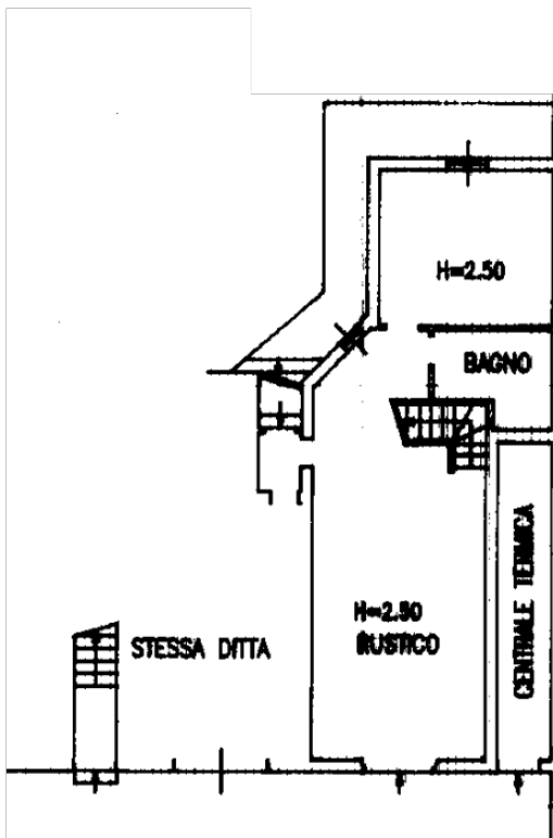
PIANO SEMINTERRATO
